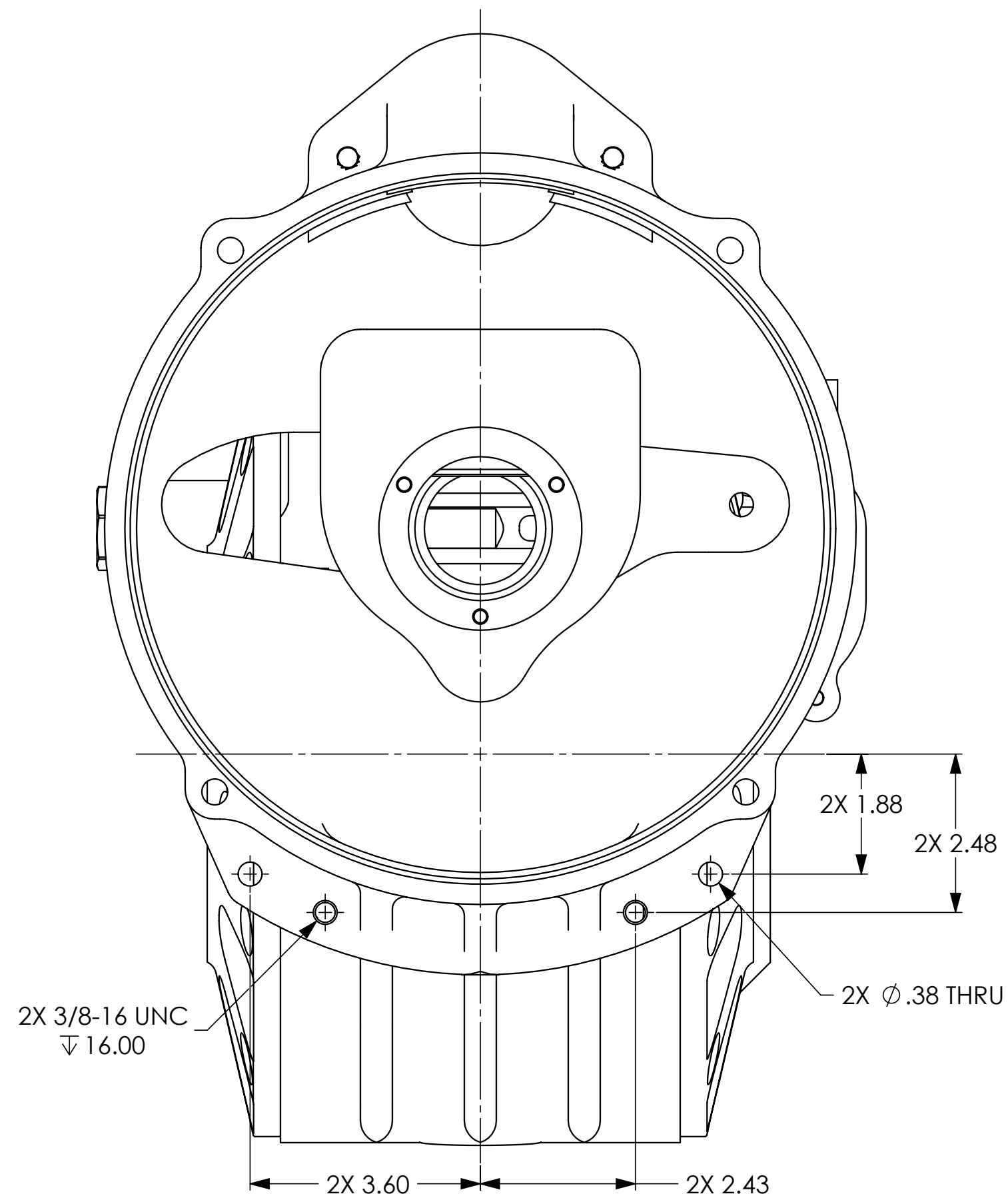
BELL HOUSING VIEW
