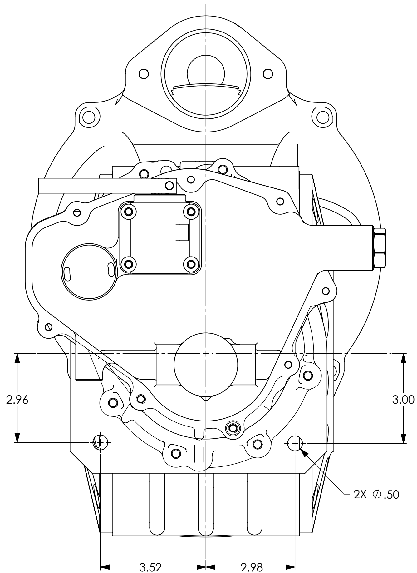
SHIFT HOUSING VIEW
