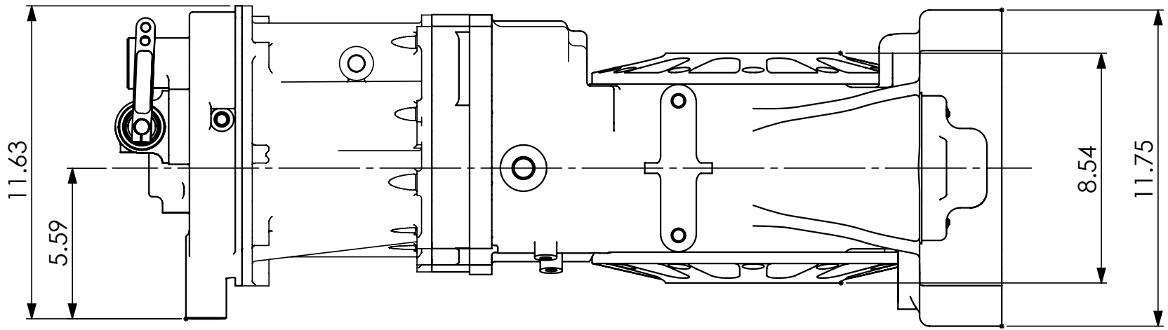
TOP VIEW
