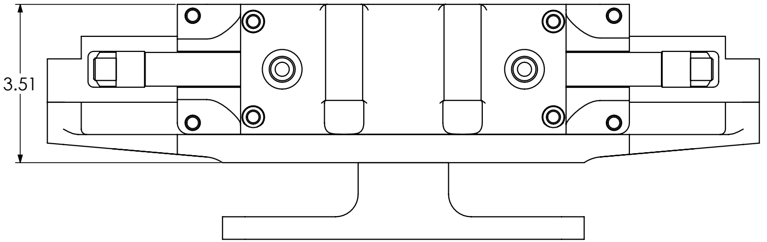
TOP VIEW
